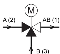
Mixing valve
