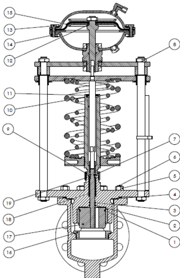
VALVE G/H1PR DN15-80
