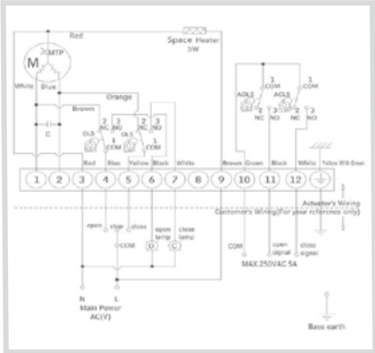
110/230 VAC On/Off type wiring diagram - for CAR-H 006-010
