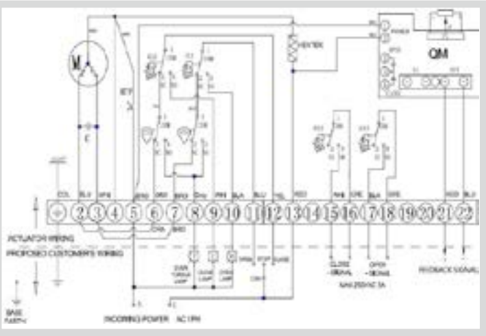
110/230 VAC CPT type wiring diagram - for CAR-H 020-S250
