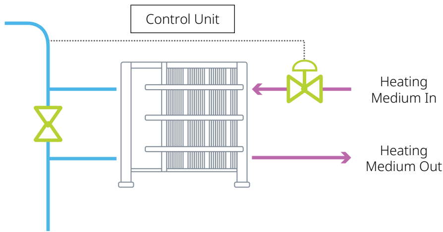
Jacket Water Heater with steam heating medium
